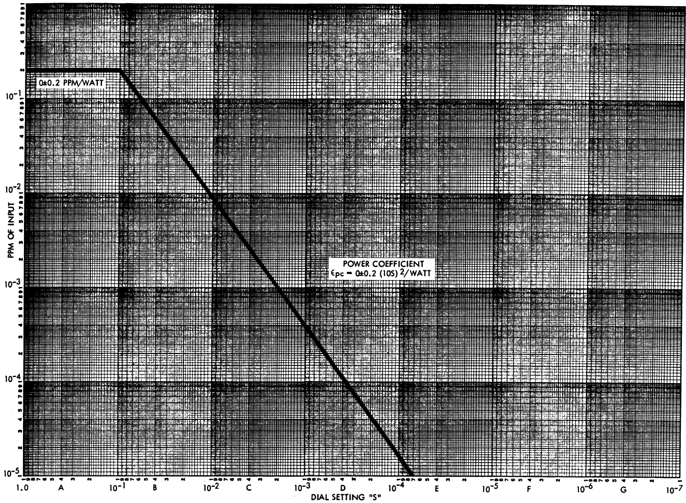
Figure 1-4. POWER COEFFICIENT
