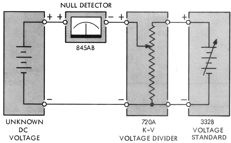
Figure 2-12. EQUIPMENT CONNECTIONS FOR SIMPLIFIED METHOD OF VOLTAGE MEASUREMENT
